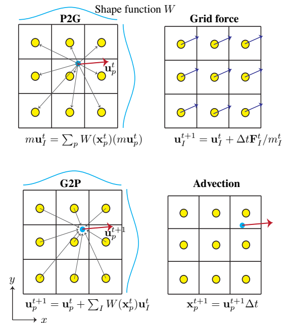
Fig. 6 Particle-In-Cell method, hybrid scheme. This example uses a cell-centered grid so information is stored at the yellow points. During simulation, momentum and weight (which can be used to get the velocity \mathbf{u}_I^t on the grid) are transferred from particles to the cell centers. In the next step, forces are applied to grid nodes to compute the new velocity \mathbf{u}_I^{t+1} . Finally, the velocity is re-transferred from the grid to particles. When particles get their new velocities, the new positions can be easily found by forward Euler integration.
