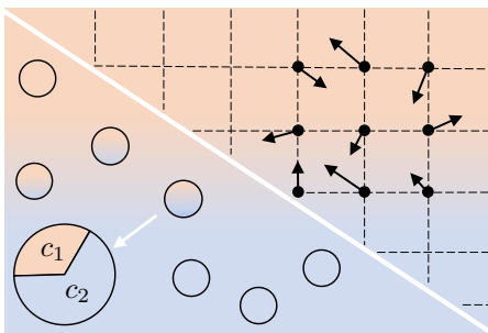
Fig. 25 Schematic diagram of mixing fluids. The lower-left part shows the fractions c_i (volume fraction, mass fraction or concentration) of different phases in each particle during the diffusion process. The upper-right part shows the 3D fluid grid; black arrows represent grid forces due to diffusion.
