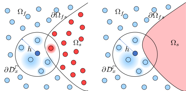
Fig. 16 Schematic diagram of fluid-solid coupling using meshless methods. Left: Discretization of the SPH approach in the coupling with materials. Fluid and solid particles both contribute to the boundary handling. \Omega denotes the domain, f denotes fluid, s denotes solid, \partial D_x denotes the surrounding spherical neighborhood. Right: Solid domain in the neighbourhood of a fluid particle represents the contribution of the boundary density value at the particle position.
