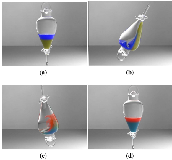
Fig. 26 Fluid extraction. From left to right, we see the change of solution due to greater solubility of the green liquid within the blue liquid than the red liquid. (a) At the beginning, the blue liquid and yellow mixture are put in a separating funnel. (b) The funnel is toppled. (c) Shaking vigorously mixes the fluids. (d) Turning the funnel upright results in a clear interface between the red liquid and a cyan mixture [169].
