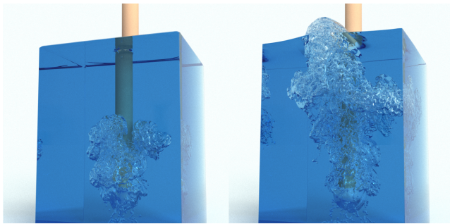
Fig. 34 The injection of gas into a glass of water [205].
