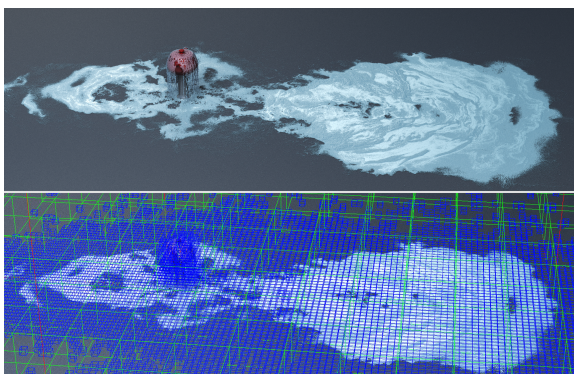
Fig. 11 A massive and sparse FLIP scene simulated using an efficient GPU parallel implementation [61] achieves one frame/second on an NVIDIA® Quadro GP100 GPU with 2 million particles and a 3360 \times 160 \times 2272 -cell grid.
