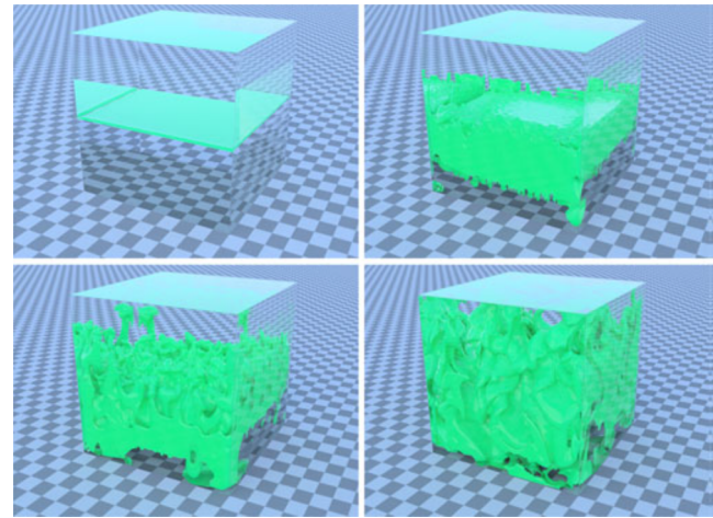
Fig. 24 Rayleigh-Taylor instability appearing at the interface between a high-density medium atop a low-density medium due to gravity [165].
