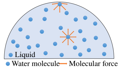
Fig. 29 Schematic diagram of surface tension. Liquids have forces between the same-kind molecules (cohesion) and between different-kind molecules (adhesion). The molecular force on the liquid surface is unbalanced, resulting in surface tension effects.
