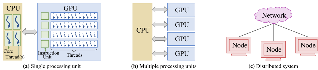
Fig. 13 Schematic diagram of different parallelization types. A single processing unit can be a multicore-CPU or a GPU. A CPU has few, but high-processing-power, cores. A GPU has weaker, but many more cores which can result in better performance for repetitive operations.
