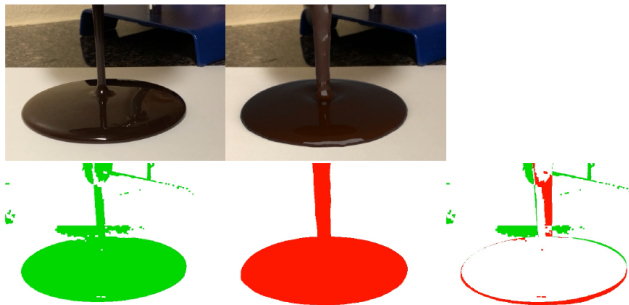
Fig. 15 The position information of the fluid is extracted from example videos as a reference (left). The 3D simulation is projected onto the screen space (middle). The difference between the two is next iteratively reduced (right) [99].
