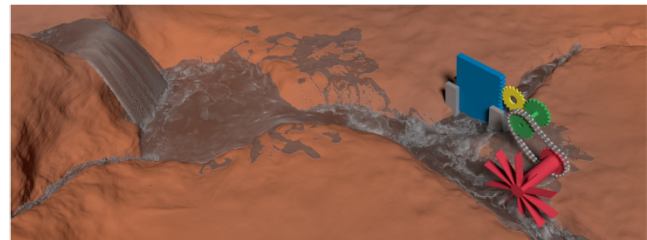
Fig. 18 SPH fluid (43.8M particles) in a terrain (50M static rigid particles) is two-way coupled with a water wheel that is connected to a gate via gears and a chain [113]. The gears, chain, and water gate are modeled with 2.3M dynamic rigid particles. Up to 90k simultaneous rigid-rigid contacts are handled.
