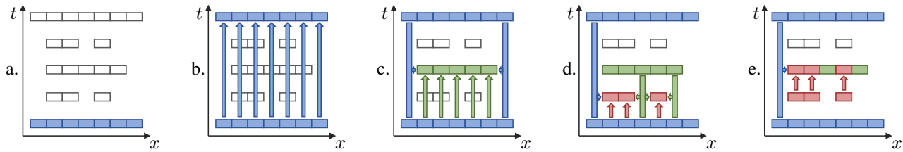
Fig. 8 Schematic diagram of the asynchronous time integration scheme in [30]. Boxes refer to discretized variables such as velocity; color represents the time step. A simulation (a) is first advanced with the largest time step (b). Next, smaller time steps are used (c, d). If values needed for computation are calculated using a larger time step, they are interpolated to match the current step size. Once the smallest time step is reached, it is used to overwrite previous results (e). The procedure is applied recursively to update all variables.
