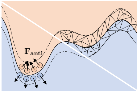
Fig. 23 Schematic diagram of non-mixing fluids. The lower-left part shows the anti-penetration force ( F_{anti} ) which is applied to particles in opposite directions along the surface normal. The embedding 3D fluid mesh can be re-tessellated in order to accommodate vertex displacement and produce changes in the interface topology.
