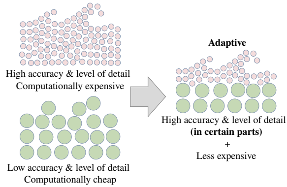
Fig. 7 Schematic diagram of particle-based adaptivity. Particle-based adaptivity adjusts particle size dynamically to reduce cost and preserve detail at the same time.
