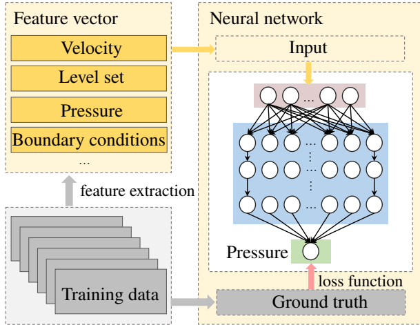
Fig. 14 Using Artificial Neural Networks (ANNs) to solve the pressure projection [95]. The network inputs feature vectors extracted from training data to output pressure as close as possible to the ground-truth one.
