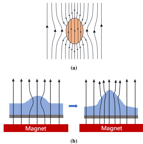
Fig. 47 Schematic representation of ferrofluids in interaction with a magnetic field. Sub-figure (a) depicts the superposition of a uniform vertical magnetic field and the magnetic field originating from an ellipsoid magnetization. There is a pronounced discontinuity in the magnetic field on the surface, most significantly at the extremities where there is a sharp escalation in the field strength. Sub-figure (b) illustrates a surface perturbation in the magnetized ferrofluid, resulting in a localized concentration of magnetic induction lines. The ferrofluid is drawn towards this bump due to a heightened field strength, which consequently enhances the gradient, amplifying the perturbation and leading to the formation of a spike.
