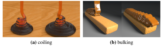
Fig. 45 Coiling and bulking effects of highly viscous fluids [299].
