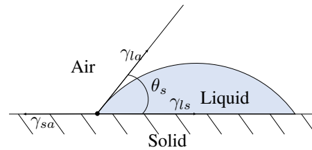
Fig. 30 Schematic diagram of stable contact angle \theta_s . \gamma_{sa} , \gamma_{la} , and \gamma_{ls} are respectively the interfacial tension coefficients for solid-air, liquid-air, and liquid-solid surfaces. When a drop of liquid rests on a solid surface in equilibrium, the angle between the solid-liquid interface and the gas-liquid interface is called the stable contact angle.
