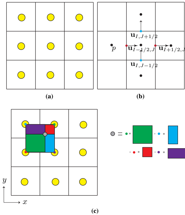
Fig. 4 Schematic diagram of Eulerian grids. (a) Collocated grid where physical quantities are stored in the cell centres (yellow points). (b) Staggered grid where different variables are stored at different locations; in this example, pressure is stored at the cell centres (black points); velocity is split into its two Cartesian components and stored at the centres of the vertical cell edges (red and blue points). Subscripts I and J denote spatial indices. (c) Using bilinear interpolation to get the value of a physical quantity at any position.
