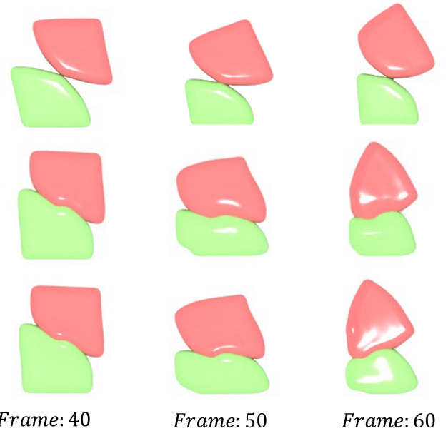
FIGURE 8 | Jelly collision. Compare the simulation results under different mesh sizes. Each row from top to bottom is the effect of low resolution, adaptive resolution and high resolution respectively.
