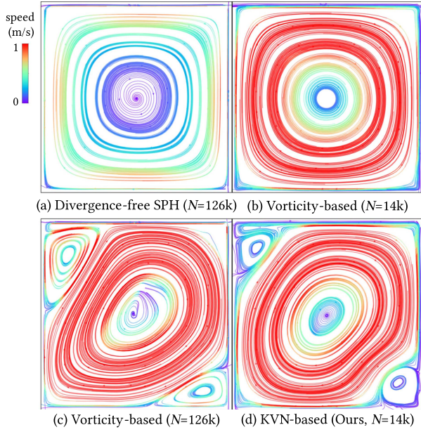
Fig. 11. Lid driven cavity visualized by streamlines. (a) Divergence-free SPH yields one central vortex using 126 k particles. (b) The vorticity-based sampling scheme using 14 k particles produces similar results, albeit with an reinforced vortex. (c) Increasing the particle count to 126 k enables vorticity-based sampling to create additional vortices. (d) Our approach produces similar results to (c) with only 14 k particles.
