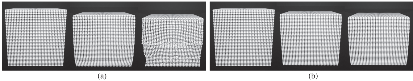
FIGURE 3 Elastic compression tests with young's modulus of E = 2 \times 10^4 KPa and a poisson ratio of \nu = 0.49 . (a) is Zhu et al. 12 method, and (b) is our method.
